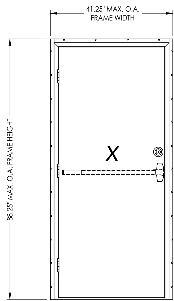
PANIC BAR EXIT DEVICE & DEADBOLT
